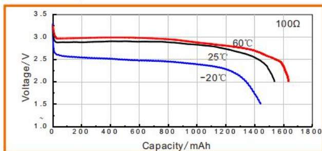
Temperature characteristics Load 100Ω
